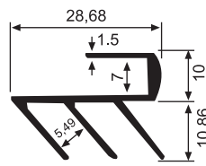
2110 B 0.250 kg/m Bombe Cam Sürgü "H" ı
