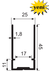
2944 0.610 kg/m Braçol Kol Fitili
