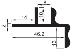
2101 0.522 kg/m Çiftli Market
