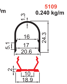
5110 PVC 20' lik Griyaj
